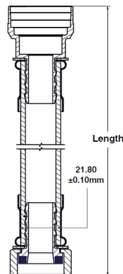
SharkBite® Water Heater Kit Dimensions
