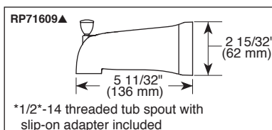
▲ Designate Proper Finish Suffix PSP-B-PTT188780 Rev. B
