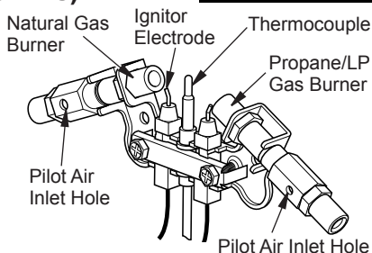
Figure 22 - Pilot Assembly
